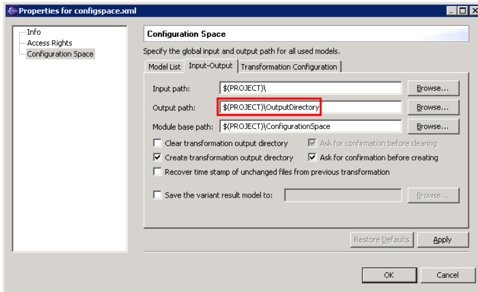
Figure 4. Transformation Output Directory
