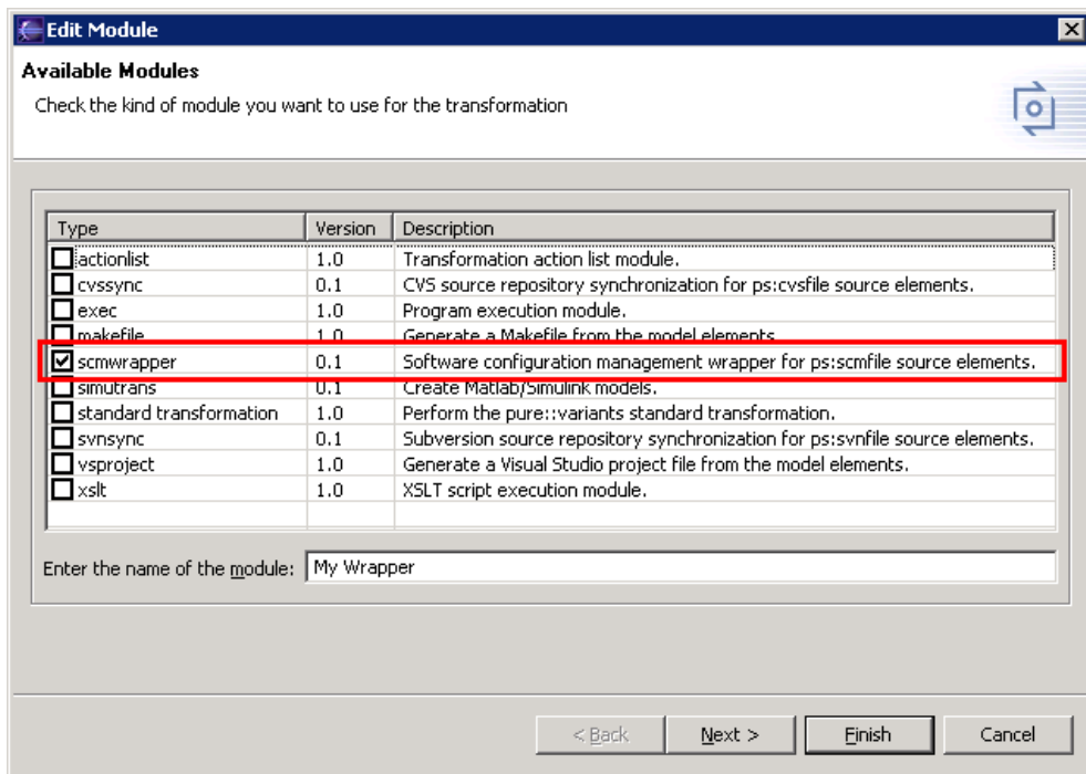
Figure 2. Available Transformation Modules
