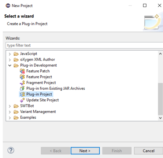
Figure 17. Plug-in Project
