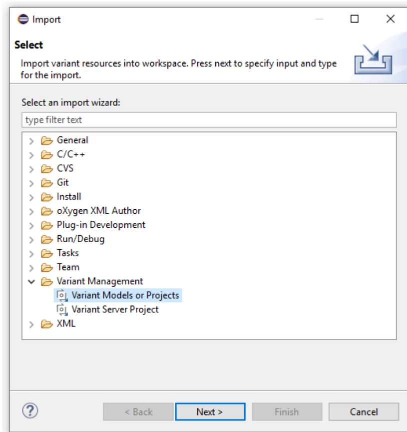
Figure 6.58. Import Dialog
