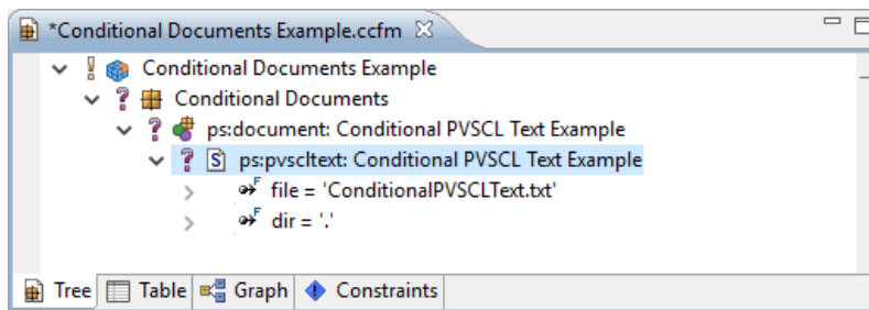
Figure 6.73. Family Model with ps:pvscltext transformation setup
