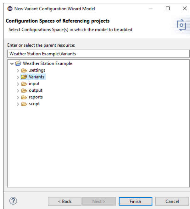
Figure 6.78. Add the new Variant Configuration Model to Configuration Spaces
