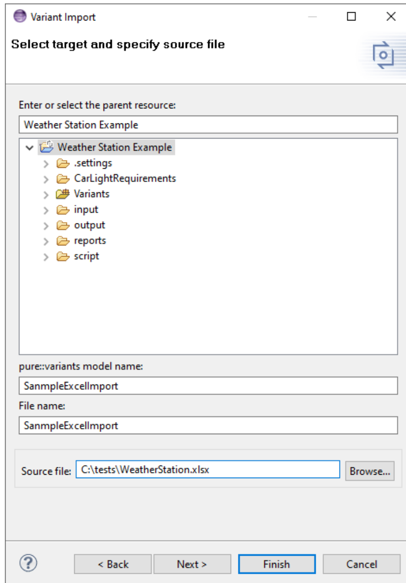
Figure 6.66. Select Target and Specify Source file
