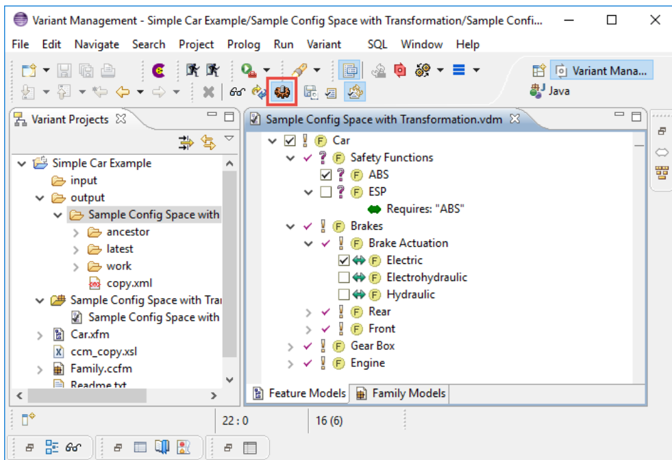
Figure 6.5. Automatically Resolved Feature Selections
