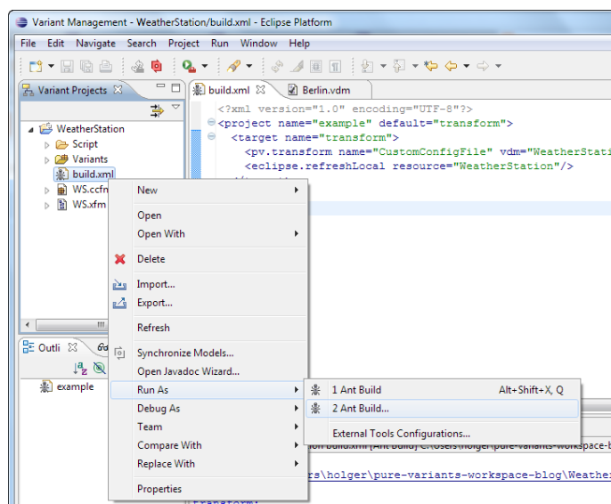
Figure 6.70. Ant Build Action
