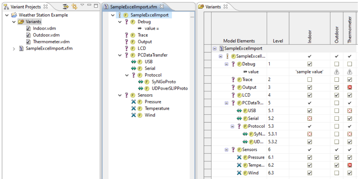
Figure 6.68. Imported Feature Model
