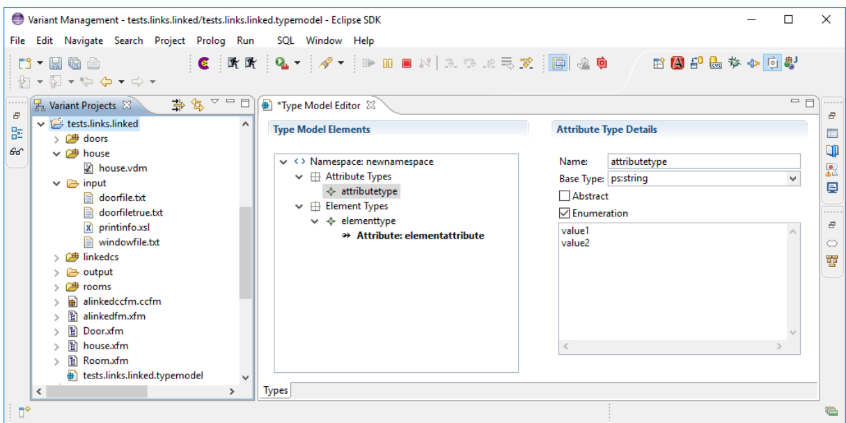
Figure 6.49. Type Model Editor Example
