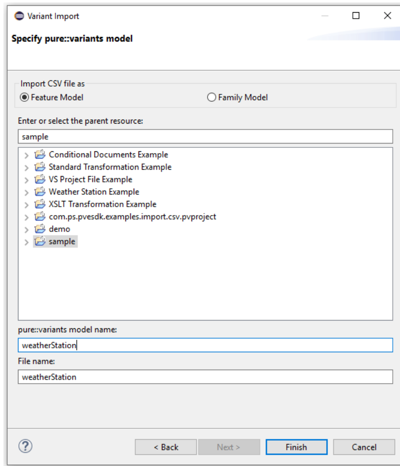
Figure 6.61. Specify pure::variants model
