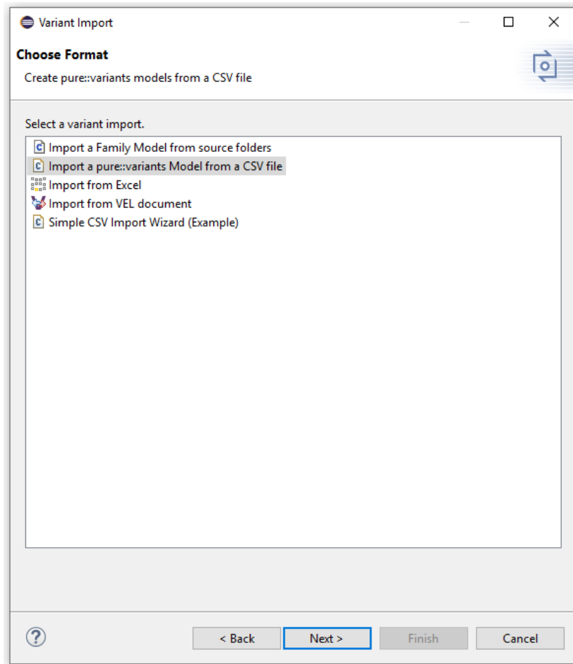
Figure 6.59. Select Variant Import Format
