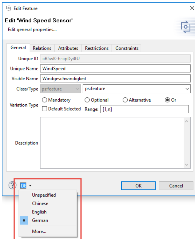
Figure 6.50. Language selection in the element properties dialog
