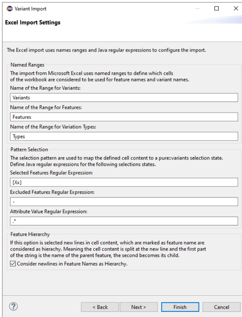
Figure 6.67. Select Pattern for feature Selection
