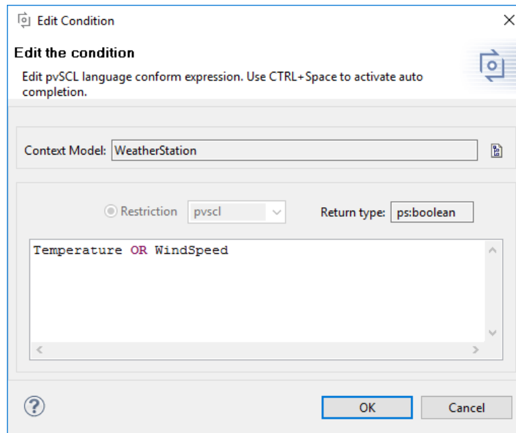
Figure 6.74. Editing pvSCL conditions or calculations
