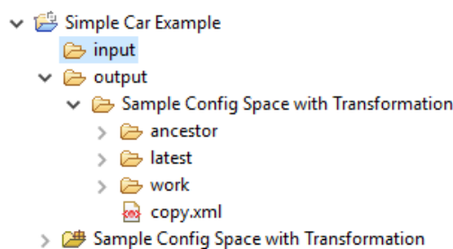
Figure 5.10. Folder Structure
