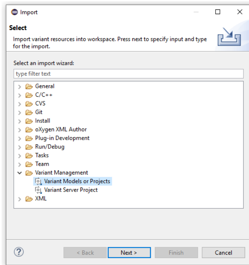
Figure 6.64. Import Dialog
