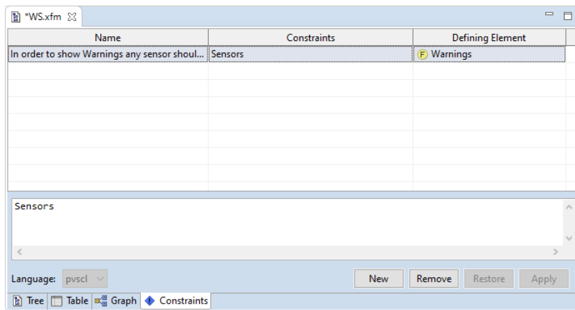
Figure 7.3. Constraints view
